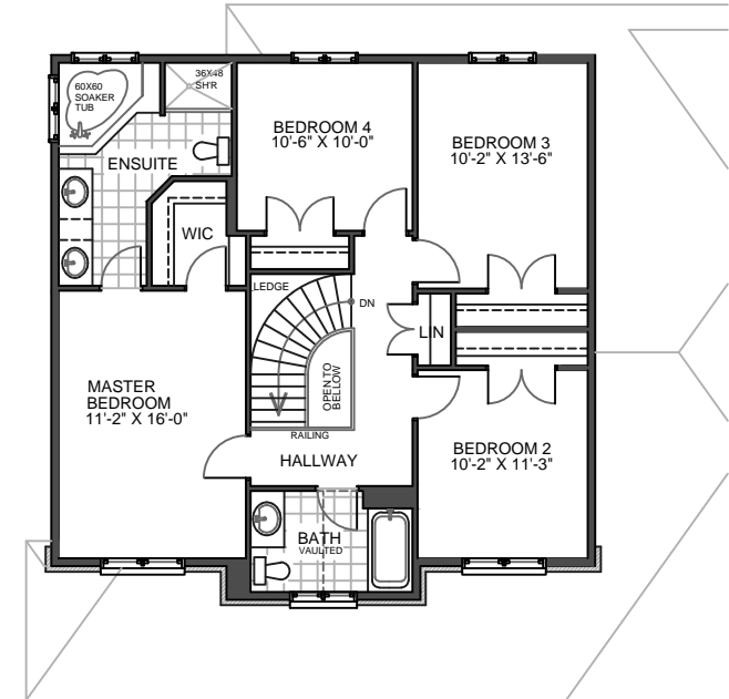
SECOND FLOOR PLAN 1,016 SQFT
