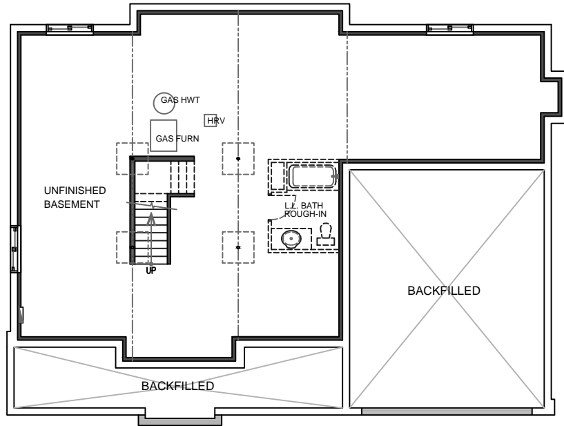
BASEMENT PLAN
