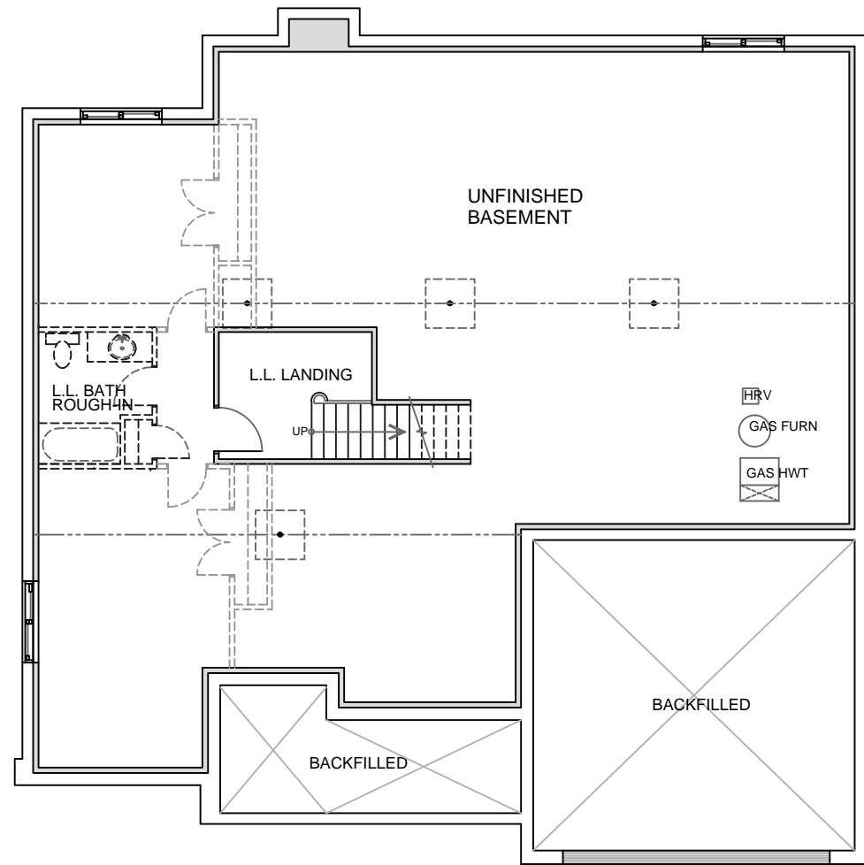
BASEMENT PLAN
