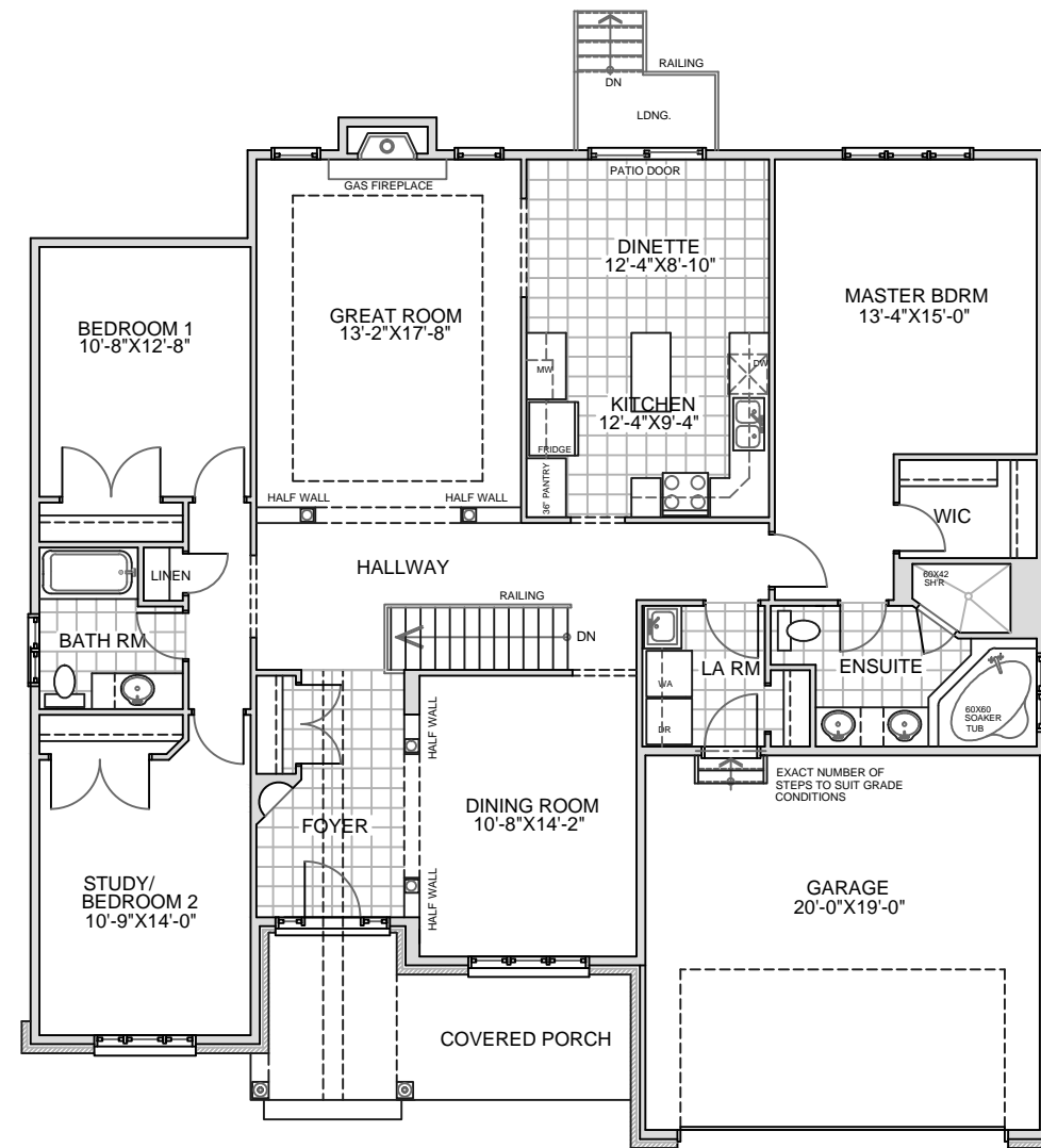
FIRST FLOOR PLAN 1,908 SQFT
