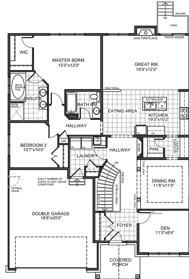
FIRST FLOOR PLAN 1,656 SQFT
