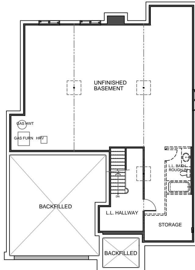
BASEMENT PLAN
