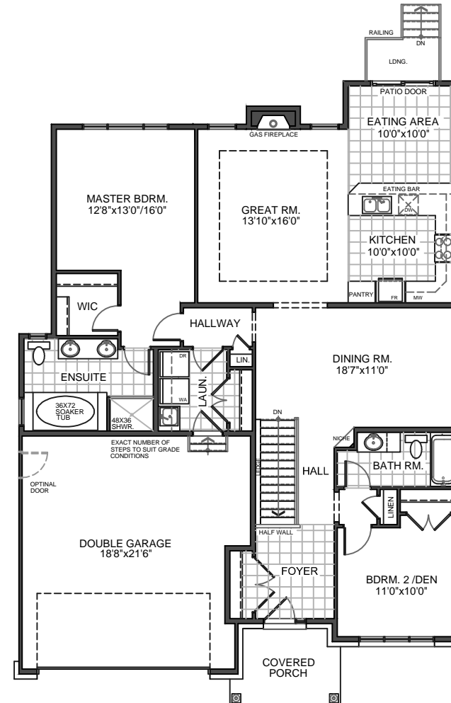
FIRST FLOOR PLAN 1,547 SQFT
