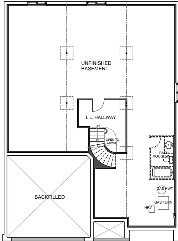
BASEMENT PLAN
