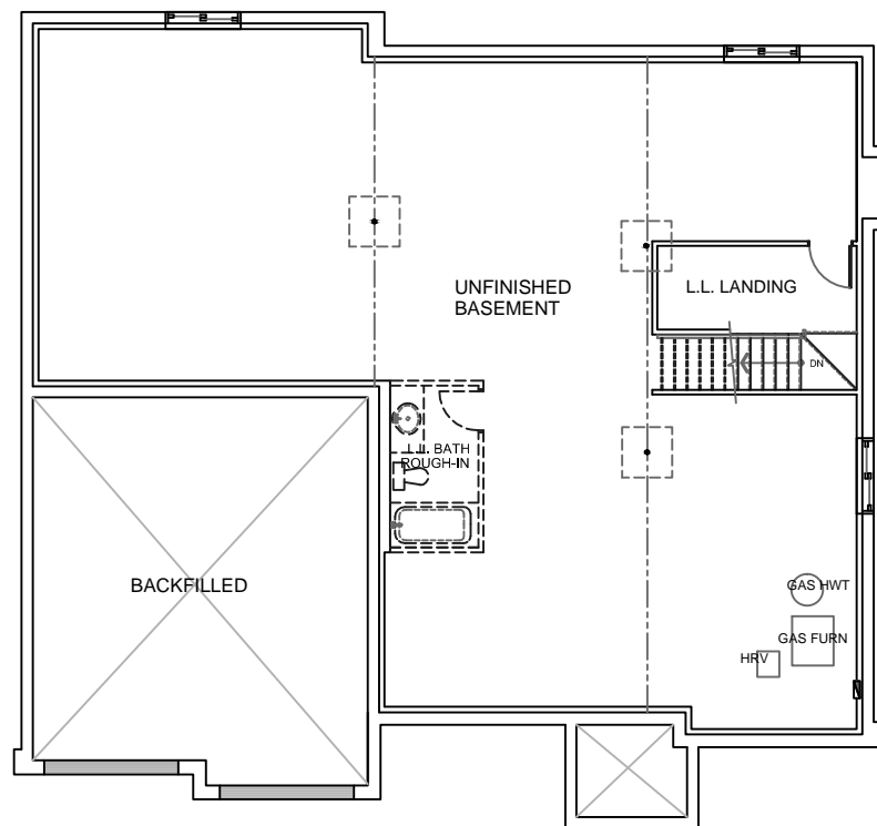
BASEMENT PLAN
