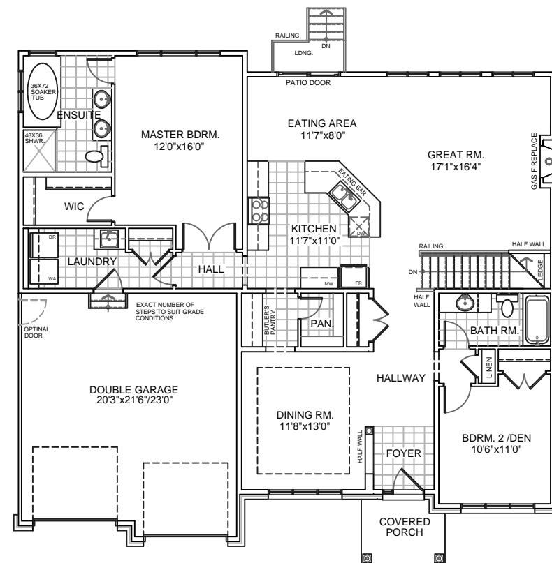
FIRST FLOOR PLAN 1,703 SQFT
