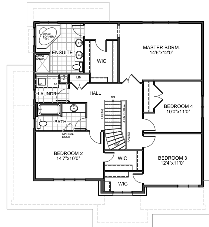
SECOND FLOOR PLAN 1300 SQFT
