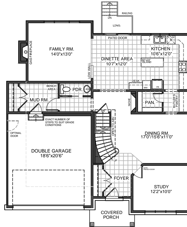
FIRST FLOOR PLAN 1196 SQFT
