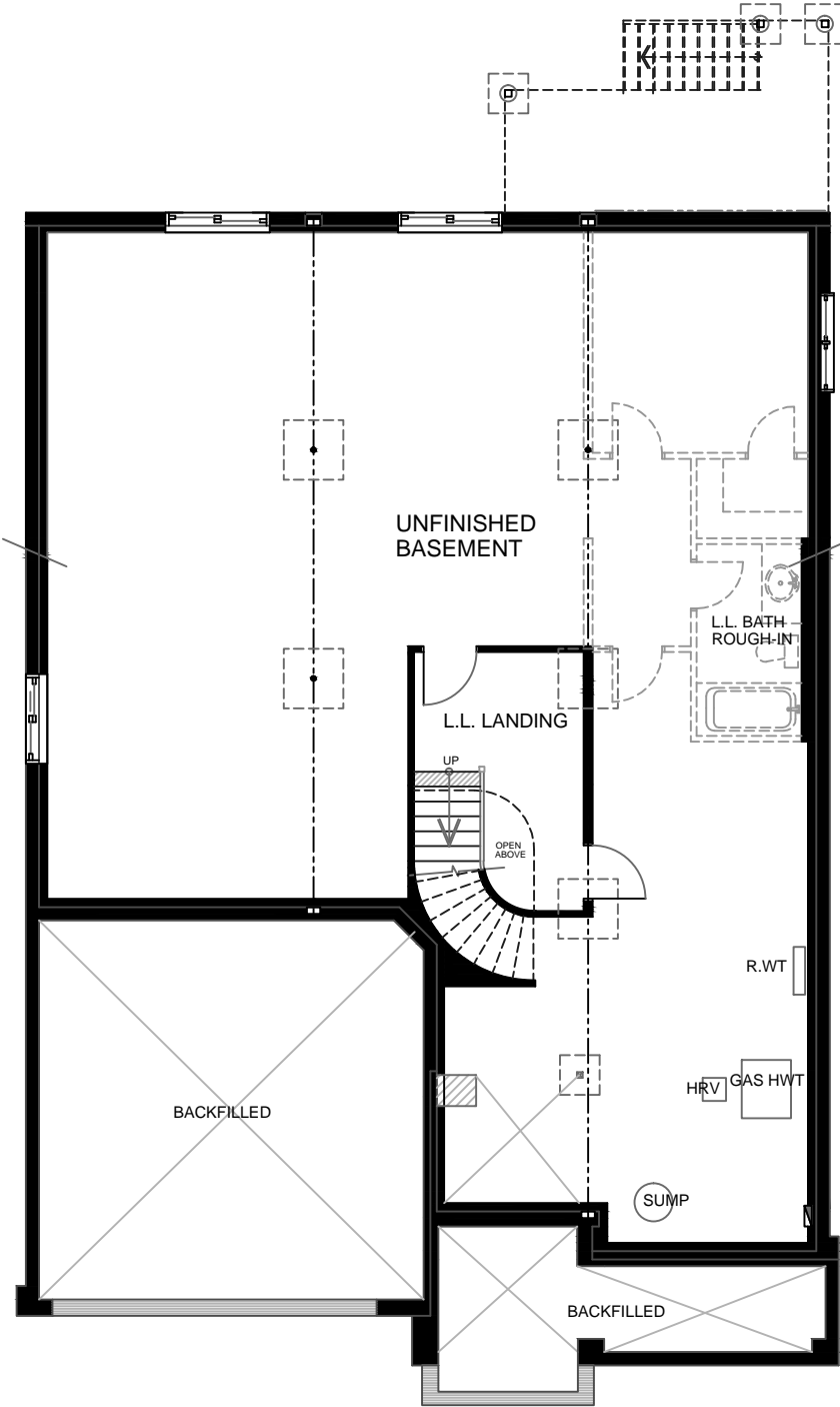
BASEMENT PLAN
