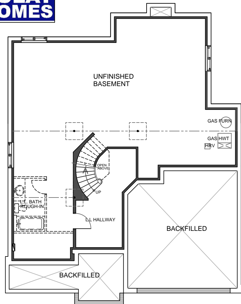
BASEMENT PLAN
