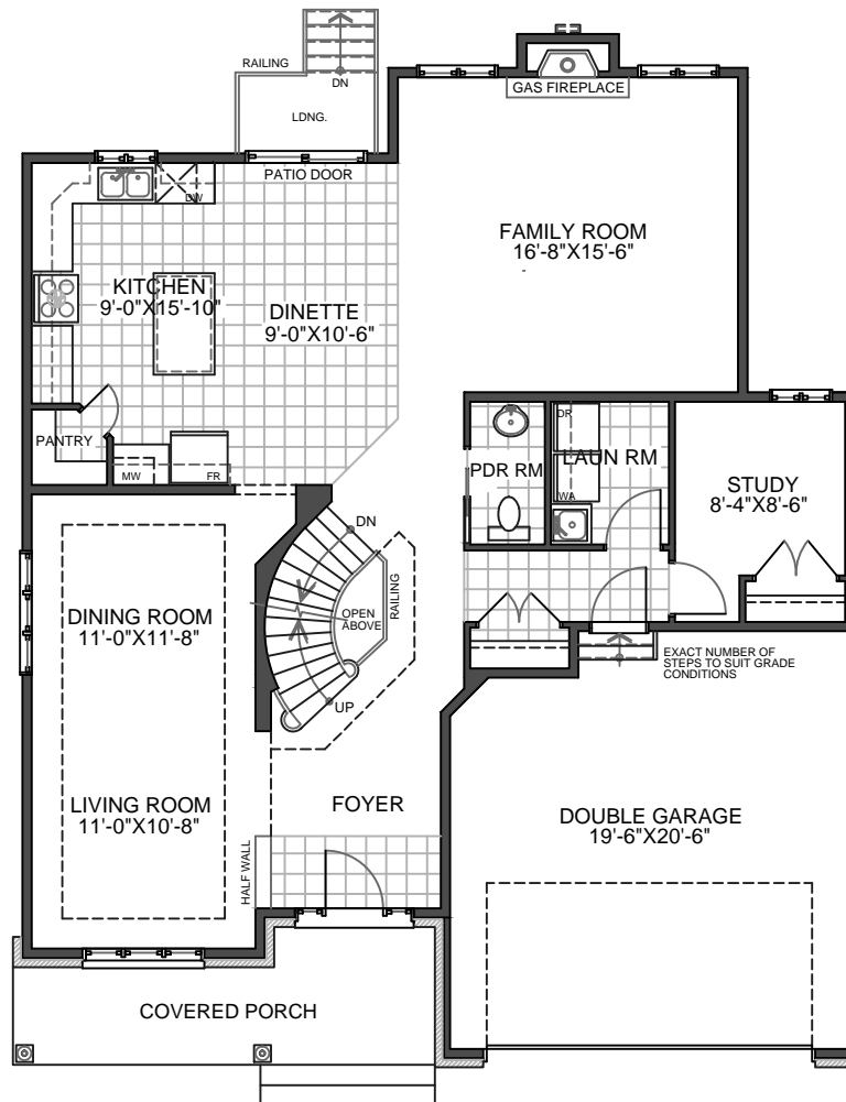
FIRST FLOOR PLAN 1,311 SQFT
