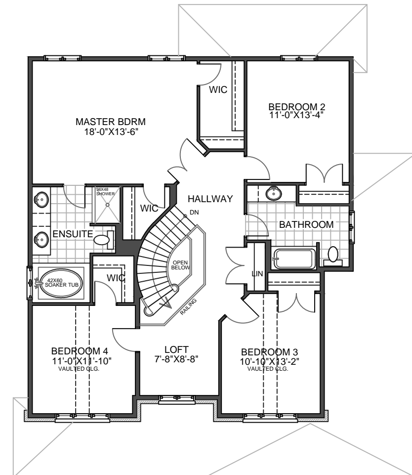
SECOND FLOOR PLAN 1,343 SQFT
