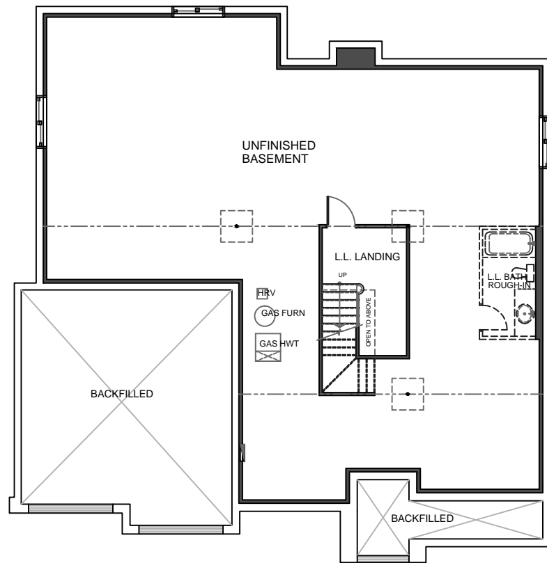
BASEMENT PLAN
