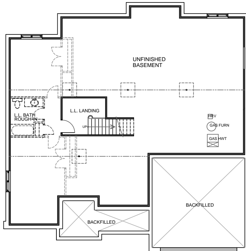
BASEMENT PLAN
