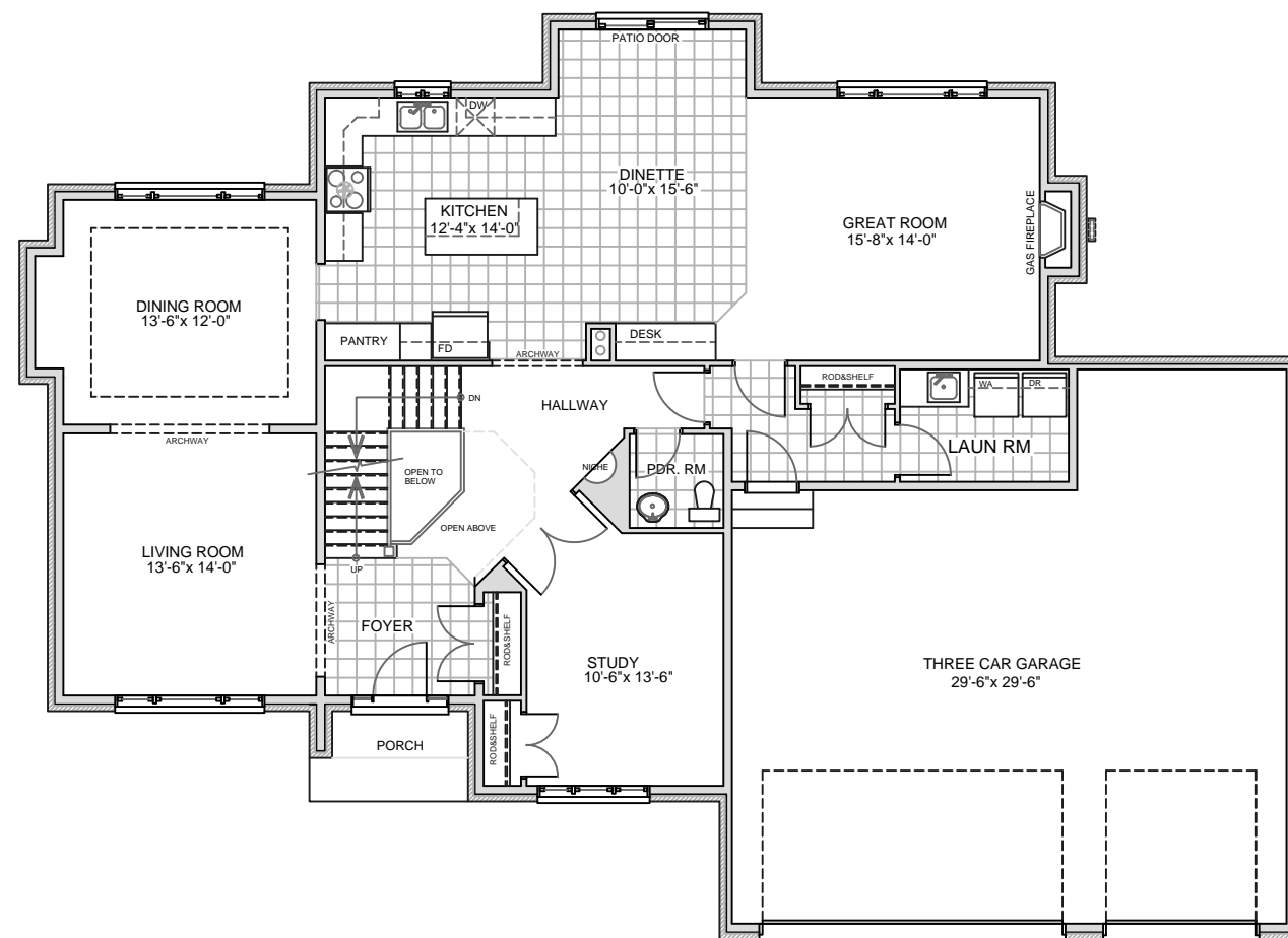
FIRST FLOOR PLAN AREA: 1596 SQFT
