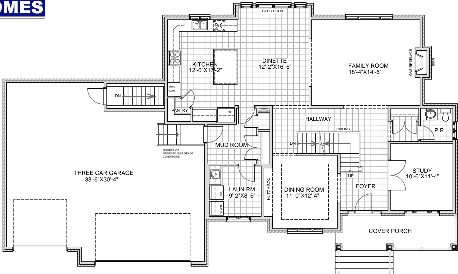
FIRST FLOOR PLAN AREA: 1,527 SQFT
