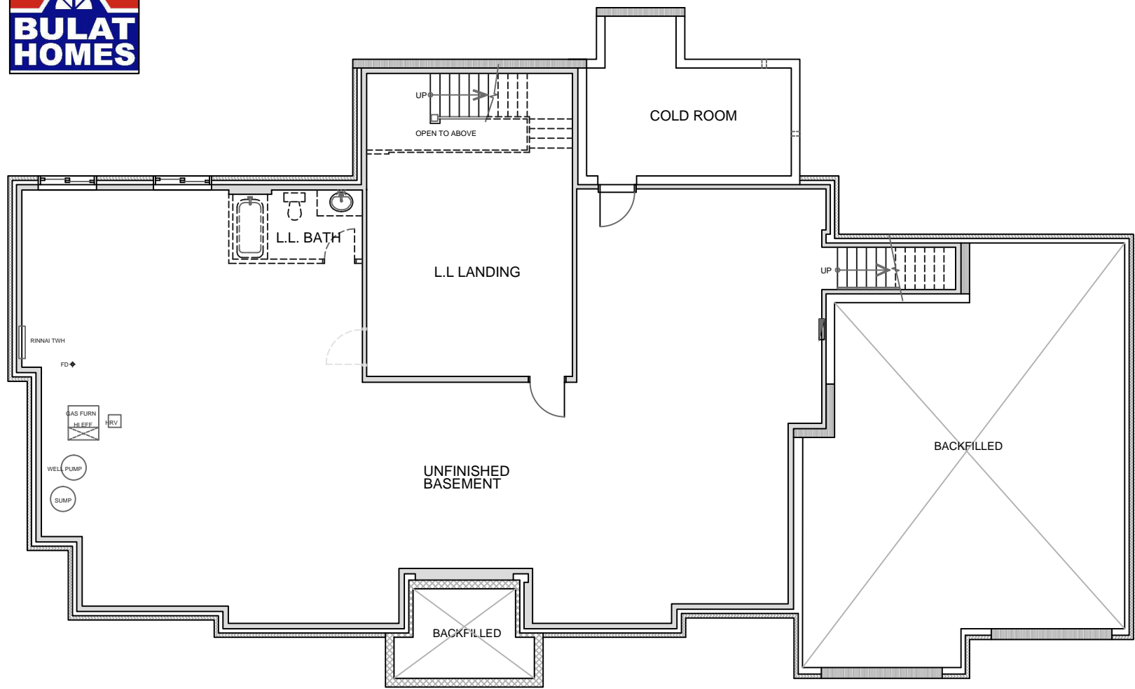
BASEMENT PLAN
