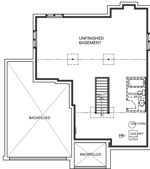
BASEMENT PLAN
