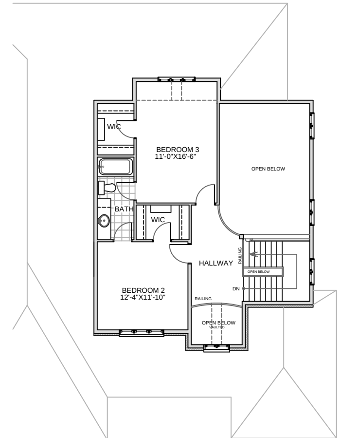
SECOND FLOOR PLAN 678 SQFT PLUS 280 OPEN SPACE
