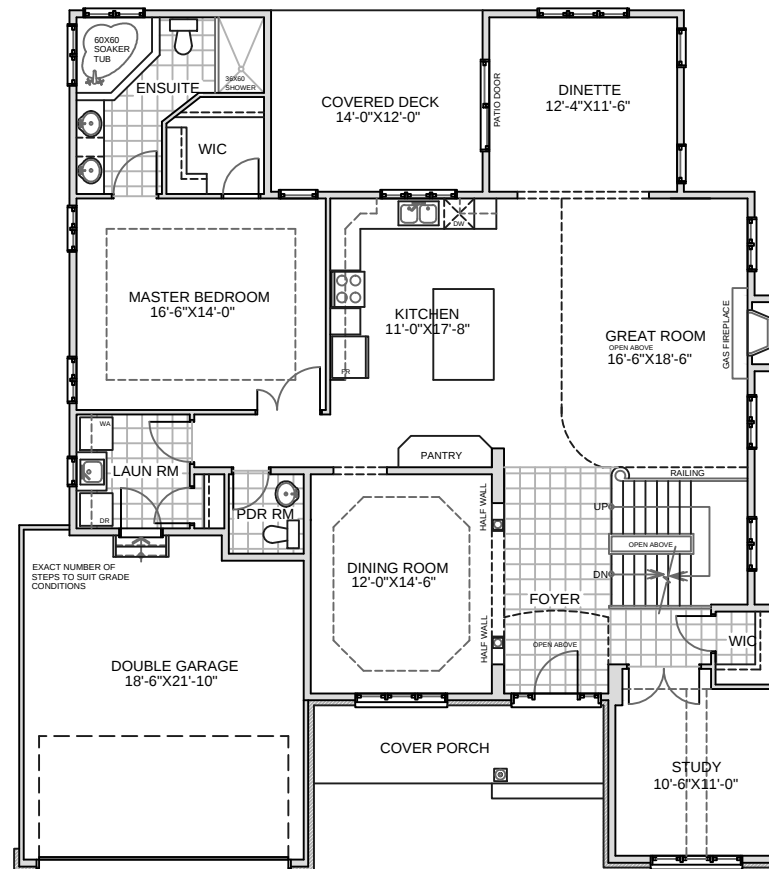
FIRST FLOOR PLAN 1820 SQFT
