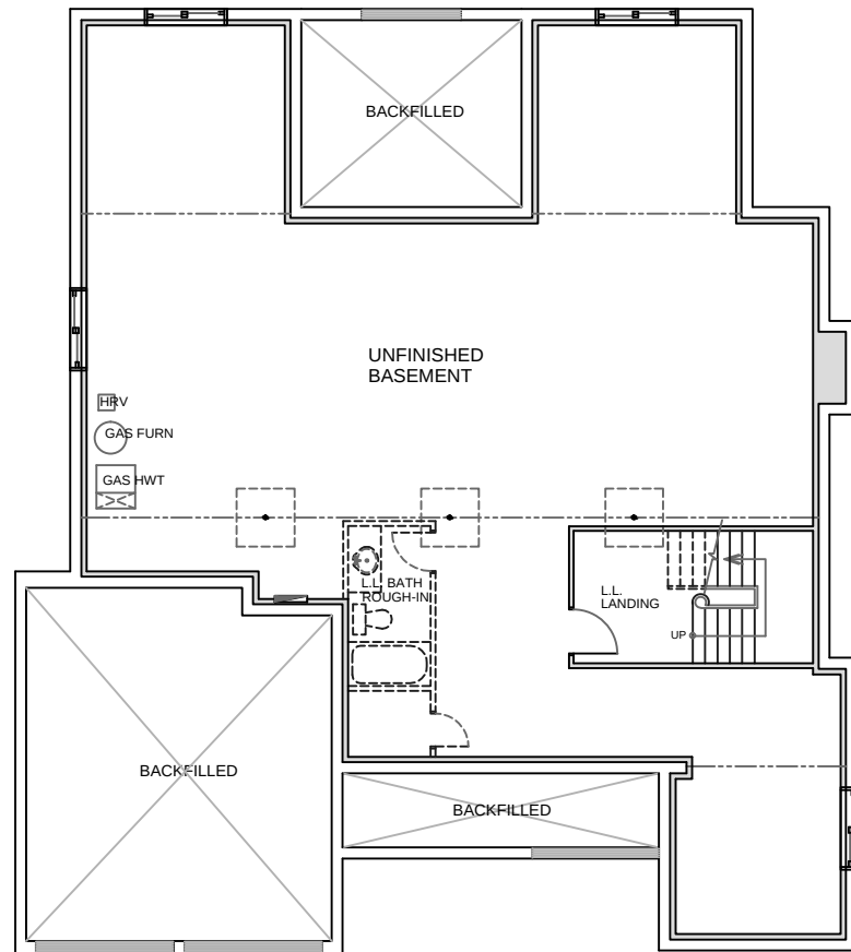
BASEMENT PLAN
