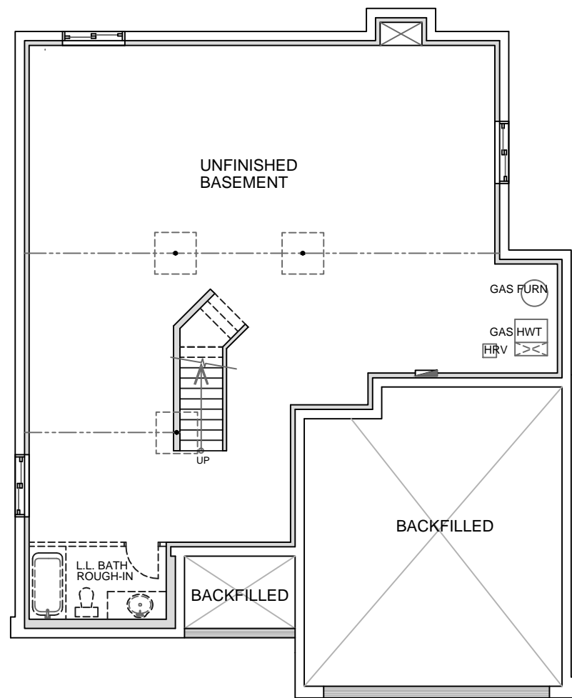
BASEMENT PLAN
