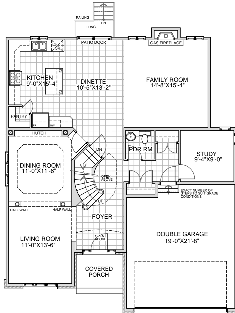
FIRST FLOOR PLAN 1,296 SQFT
