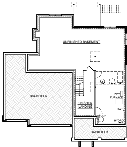
BASEMENT PLAN 105 SQFT
