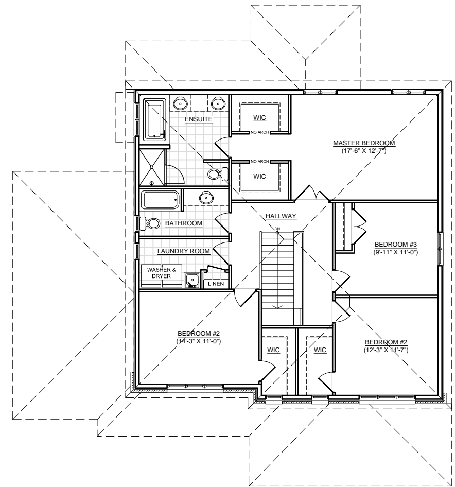
SECOND FLOOR PLAN 1,300 SQFT
