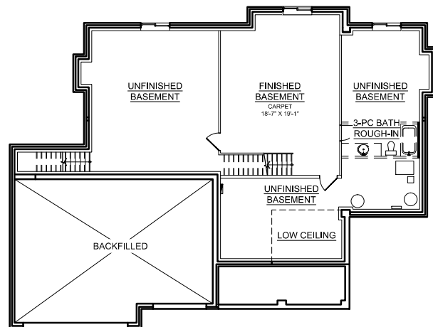
BASEMENT PLAN 414 SQFT
