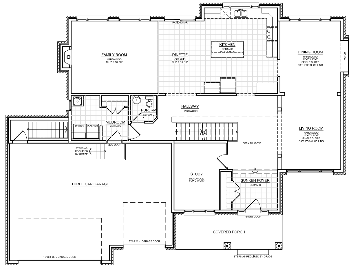
FIRST FLOOR PLAN 1,678 SQFT
