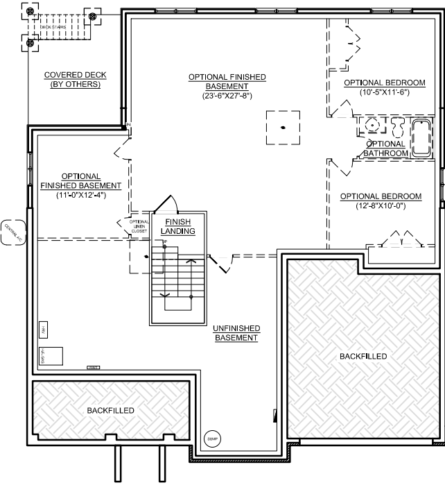
BASEMENT PLAN 28 SQFT
