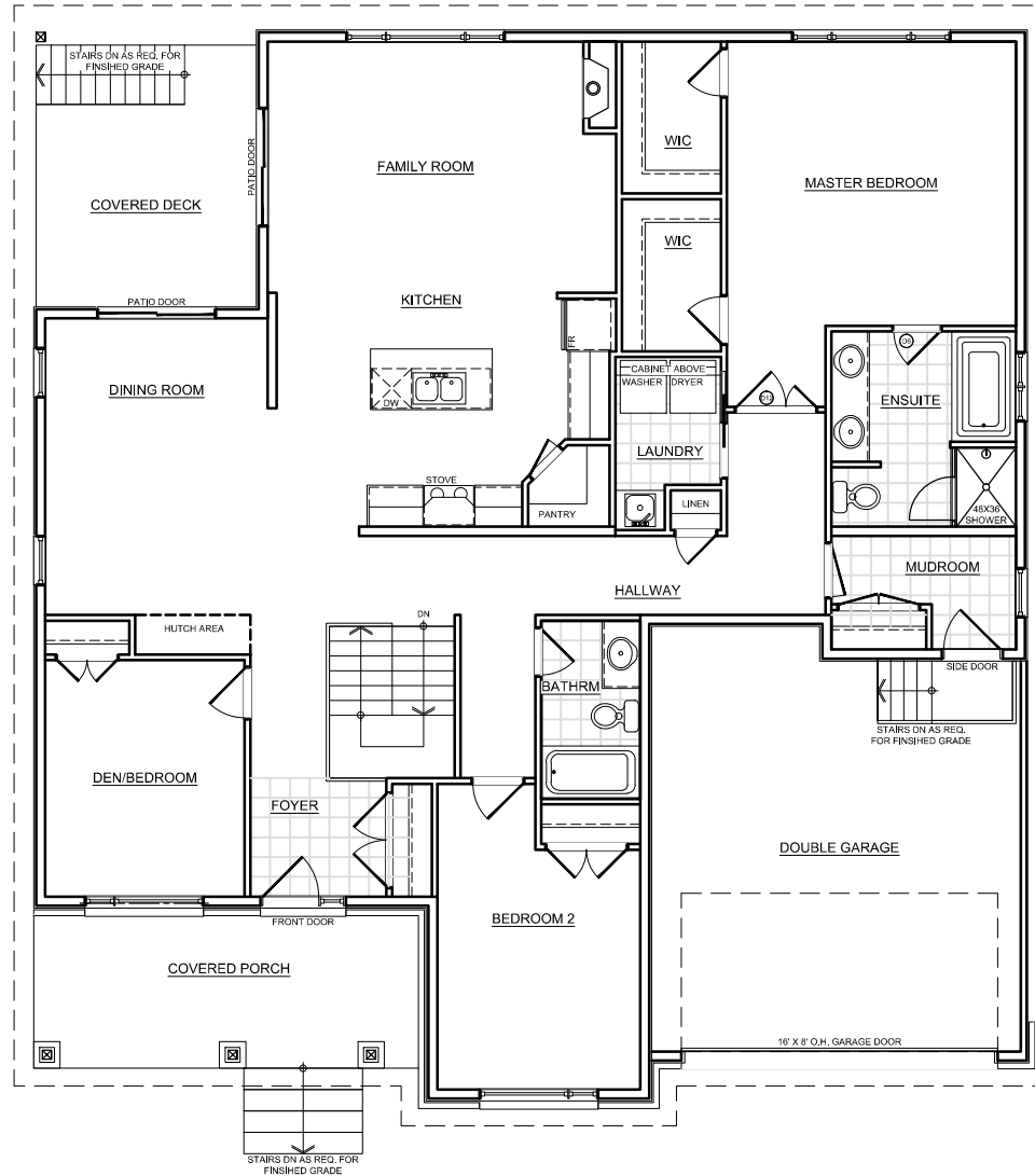
FIRST FLOOR PLAN 1,907 SQFT
